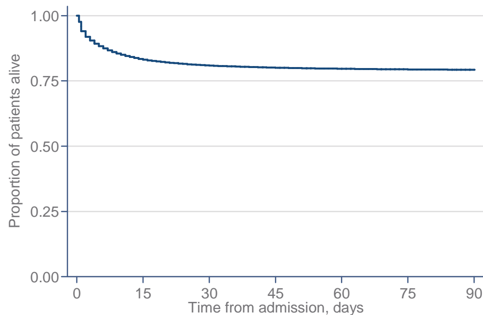
Kaplan-Meier survival plot
